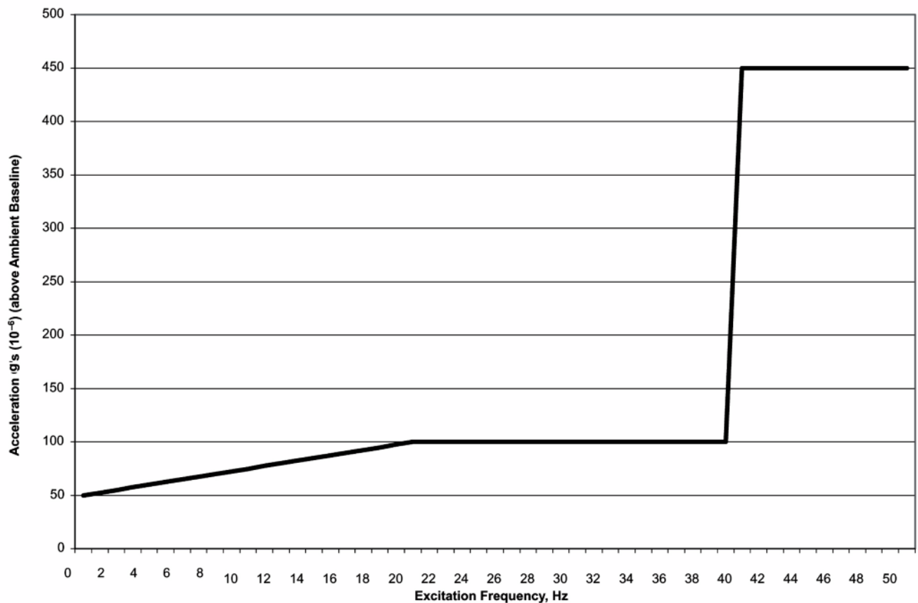
Illustration 5-9: 1.5T LCC Magnet Steady State Vibration Specifications
