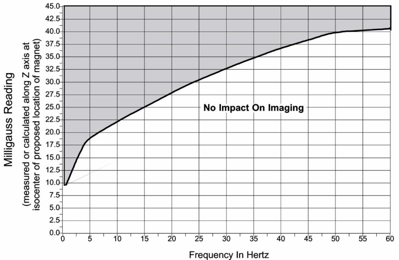
Illustration 5-8: Allowable Milligauss VS Line Frequency For AC Equipment
